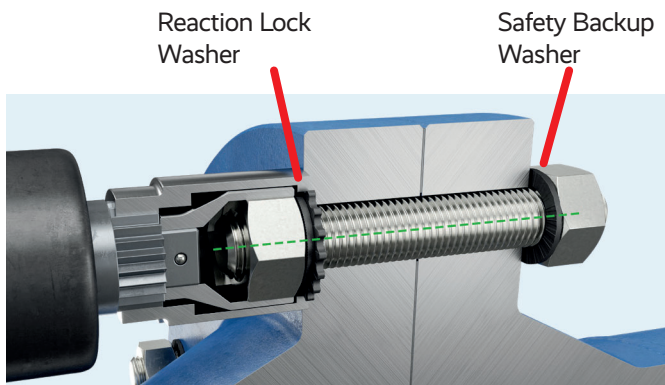
Use of Safety Backup Washer in combination with a Reaction Lock Washer.
